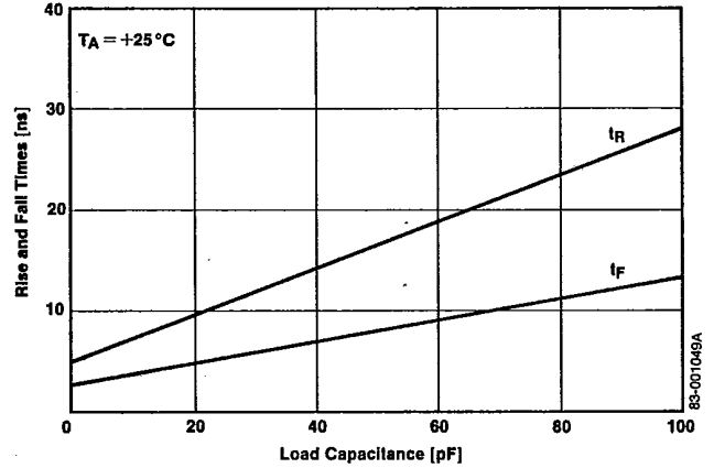
Rise and Fall Times vs Load Capacitance
